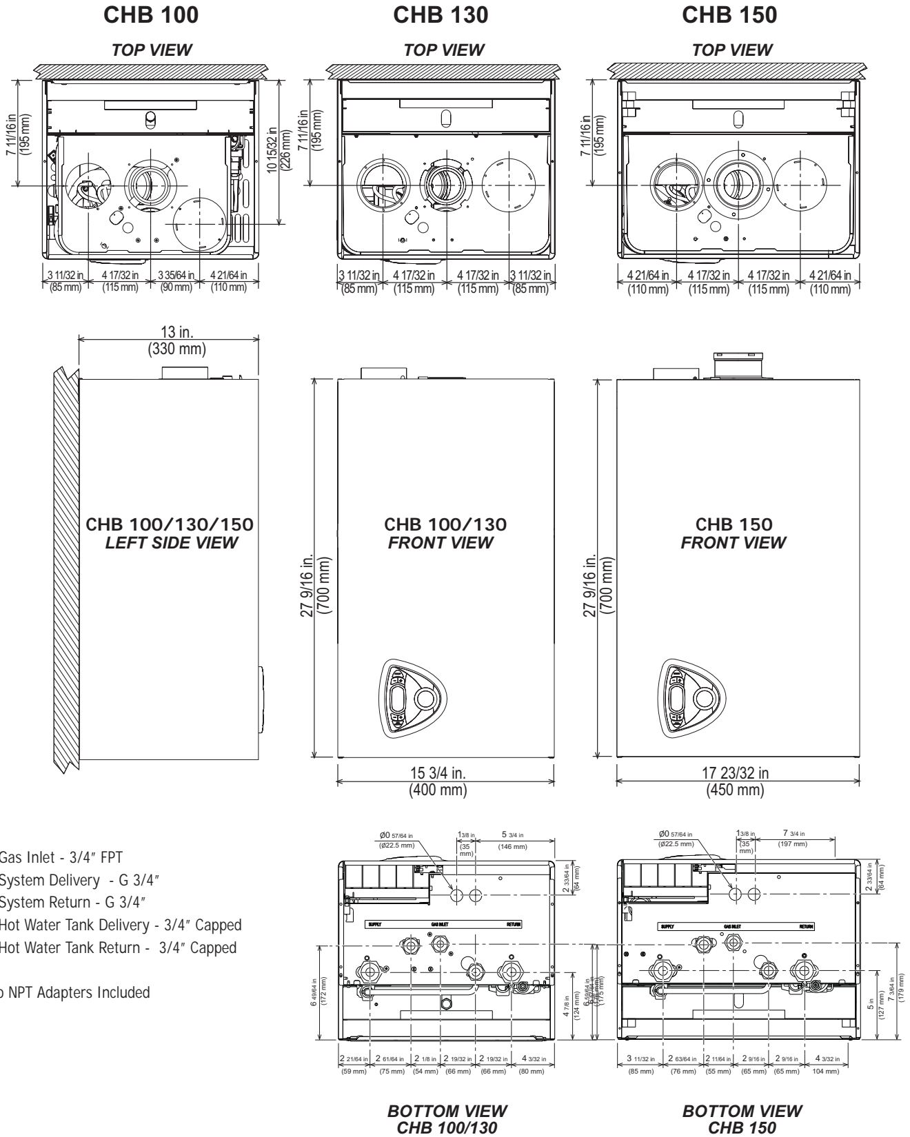
Figure 1 - Overall Dimensions
