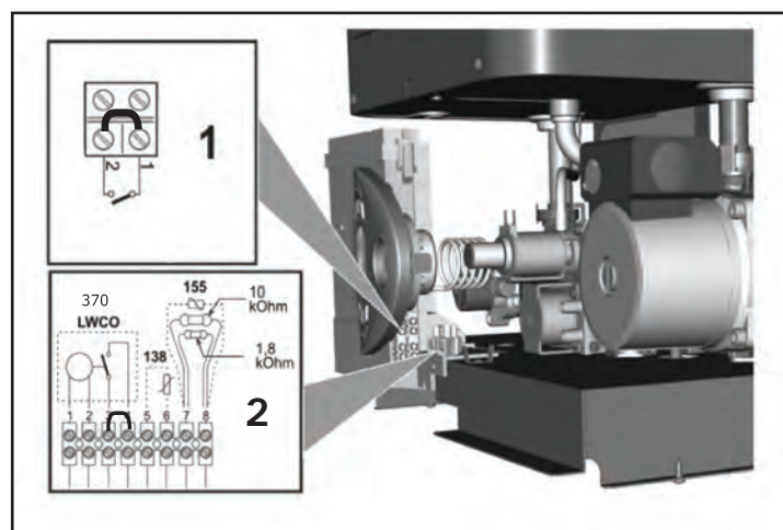
Figure 18 - Bornier
