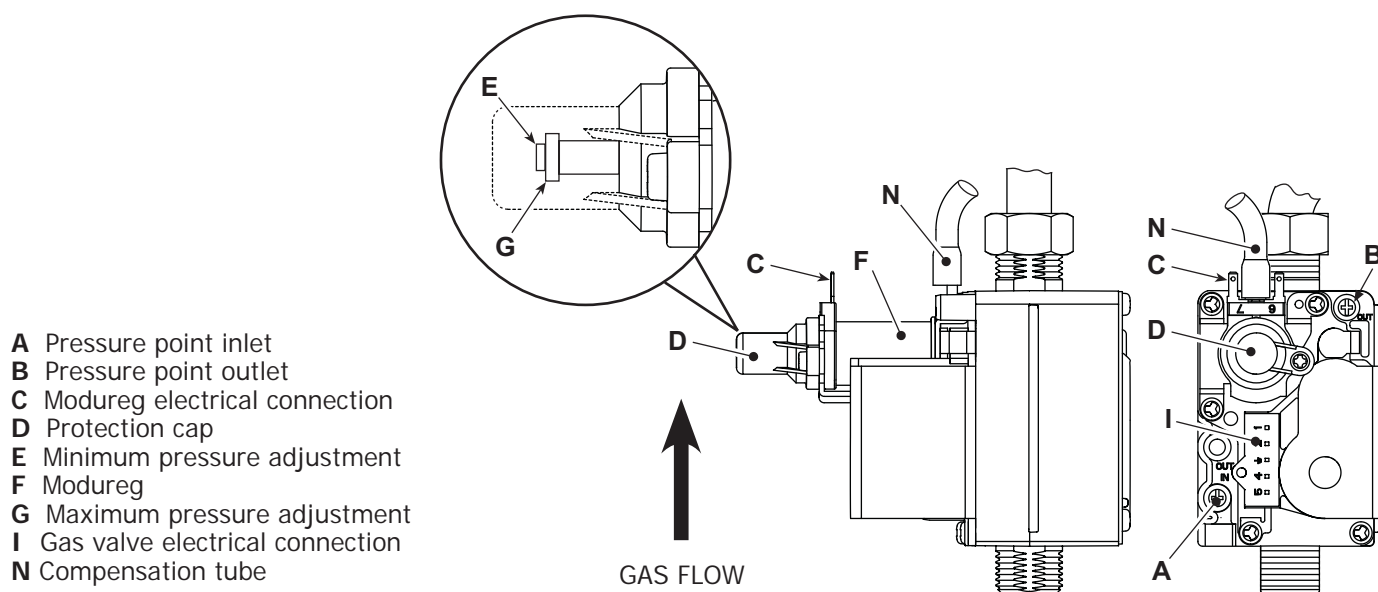
Figure 20 - Gas Valve
