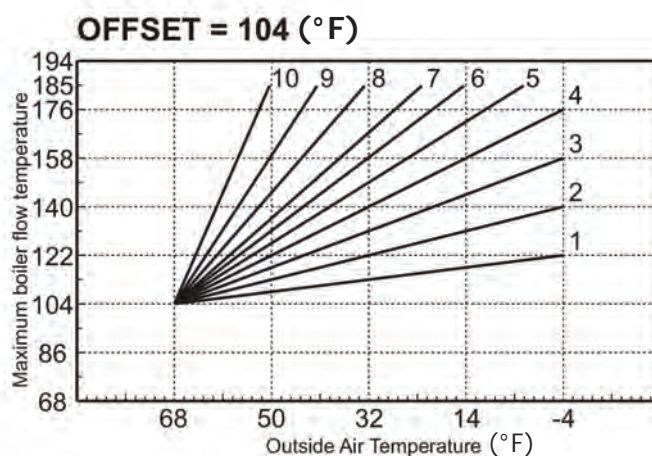
- Compensation curves
