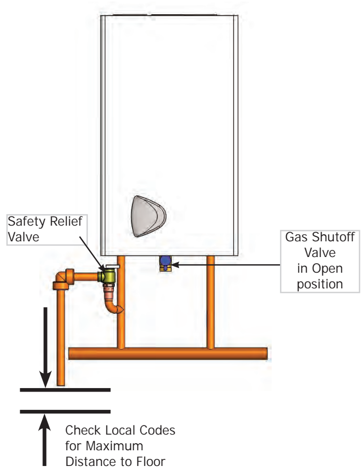
Figure 9 - Safety Relief Valve Discharge Piping
