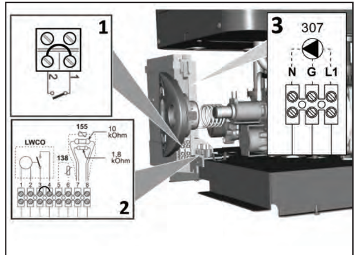
Figure 18 - Terminal Block
