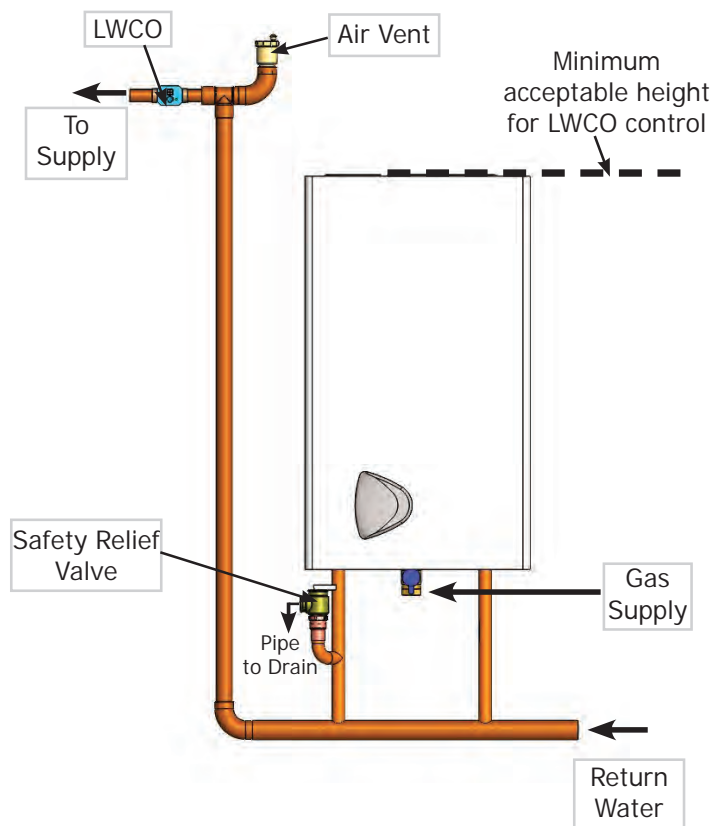
Figure 10 - LWCO Suggested Probe Location
