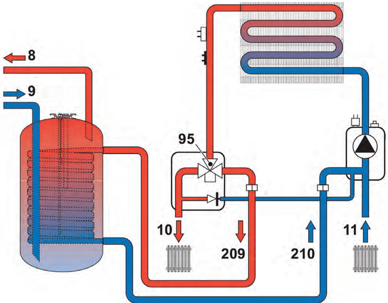
Figure 11 - Tuyauterie hydronique
