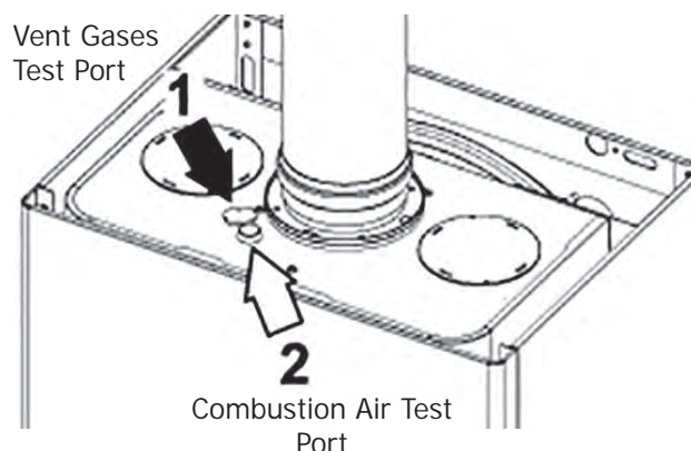
Figure 19 - Test Ports
